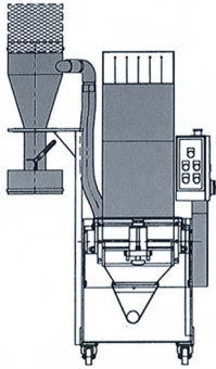
Basic Machine with Granule Discharge to Bin
